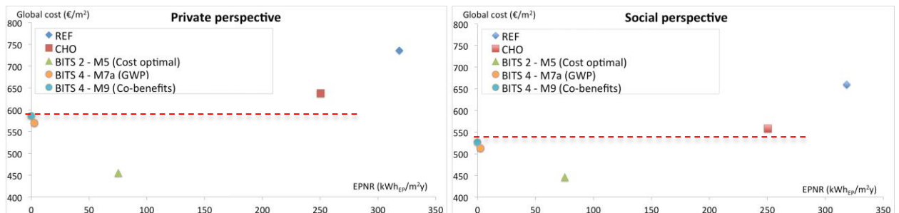
Fig. 4. Life cycle costs evaluation graphs for the best solutions of each assessment carried out.
